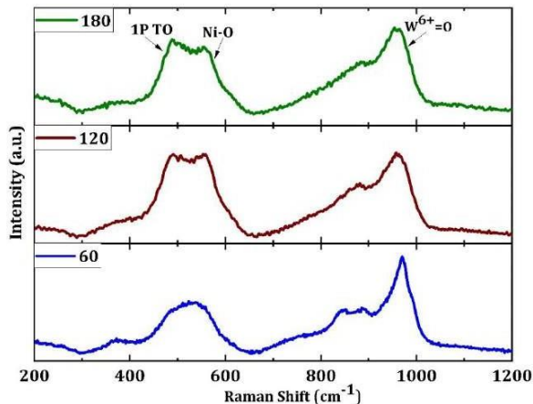
Fig. 5. Micro-Raman Spectra of Ni-W thin films deposited at 60, 120 and 180 minutes.
